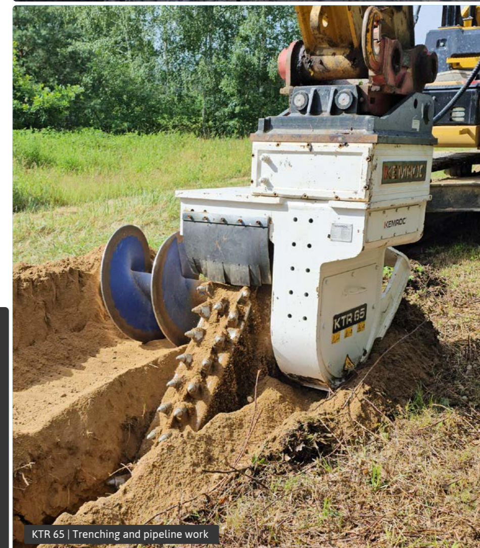
KTR 65 | Trenching and pipeline work
